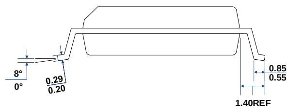
LEFT-SIDE VIEW
