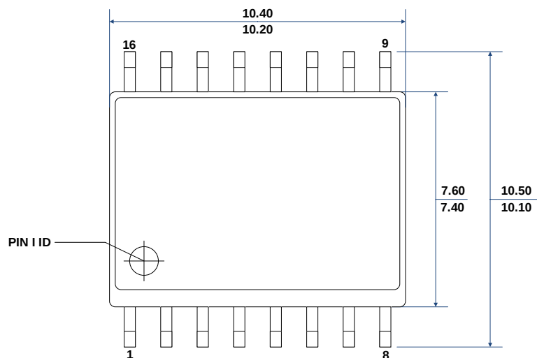
TOP VIEW
