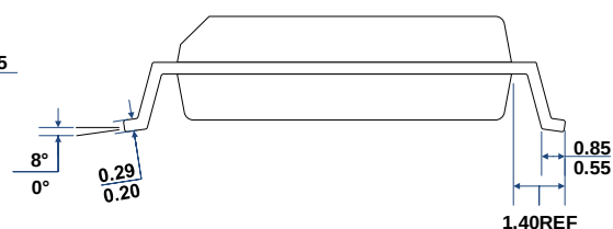
LEFT-SIDE VIEW
