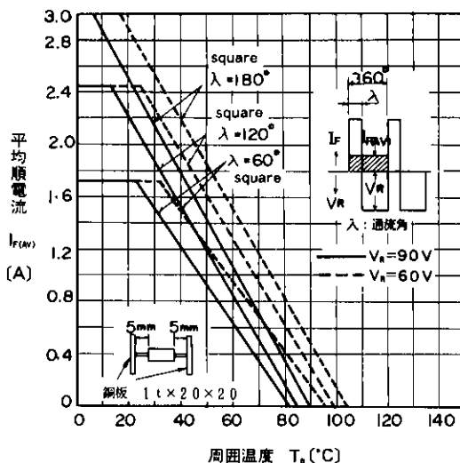
I_{F(AV)}-T_A Characteristics
