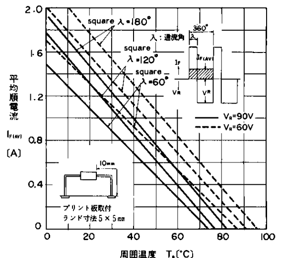
I_{F(AV)}-T_A Characteristics
