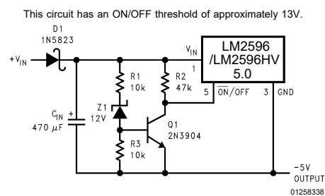
FIGURE 23. Undervoltage Lockout
