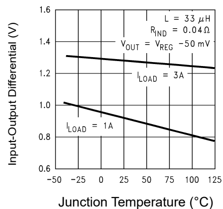
Figure 6: Dropout Voltage
