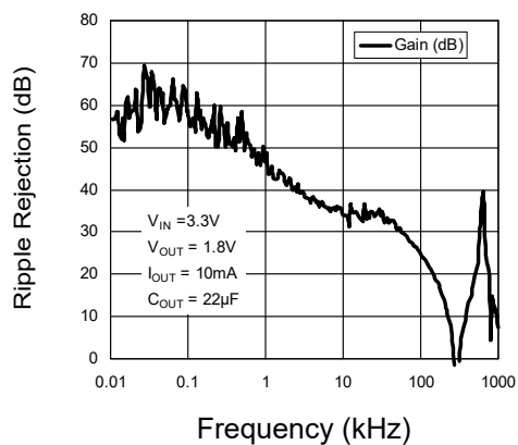
Figure 15: Ripple Rejection ( I_{OUT}=10mA ) vs. Frequency
