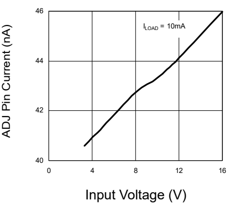
Figure 4: Adjust Pin Current vs. Input Voltage
