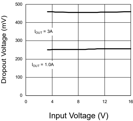
Figure 1: Dropout Voltage vs. Input Voltage
