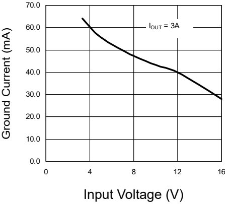
Figure 2: GND Pin Current vs. Input Voltage
