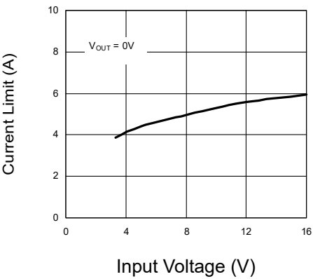
Figure 6: Short-Circuit Current vs. Input Voltage
