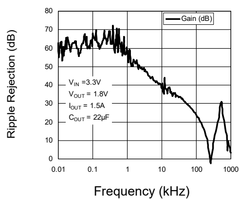
Figure 16: Ripple Rejection ( I_{OUT}=1.5A ) vs. Frequency
