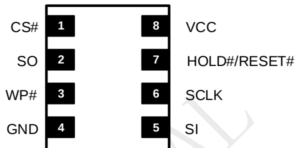
8-Pad WSON (6x5/8x6mm) and USON(4x4/3x2mm)
