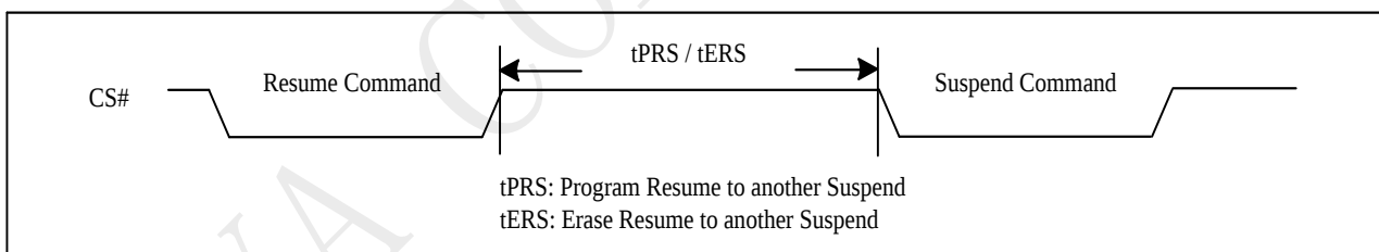
Figure 10-41 Resume to Suspend Latency
